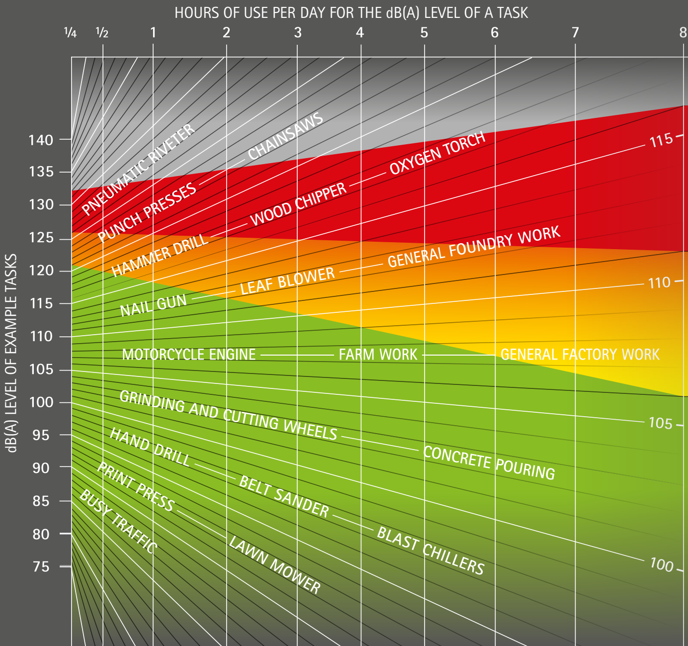
This chart uses decibel levels of work place environments and has example tasks to give an idea of real world sound levels. It includes the amount of time that you could potentially spend in a particular environment. This chart is for general guidance only and should not be considered a substitute for a full risk assessment.
